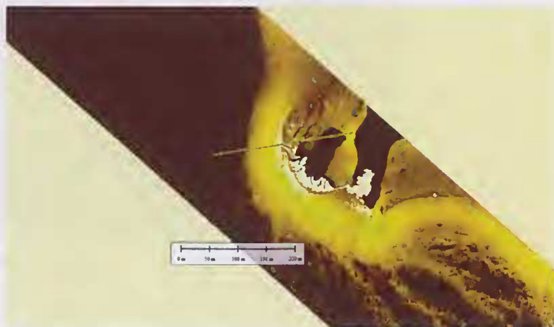
Figure 7. Transect 3, northern margin of South Turtle Reef. A) High resolution digital photograph of the lower portion of the transect from the lagoon and across the reef-front ramp and a wide lower-littoral flat at the water's edge. B) Contour map of the same area derived from LIDAR data. C) NDVI image of the same area showing areas of intense photosynthetic activity. [Images: courtesy Airborne Research Australia].
